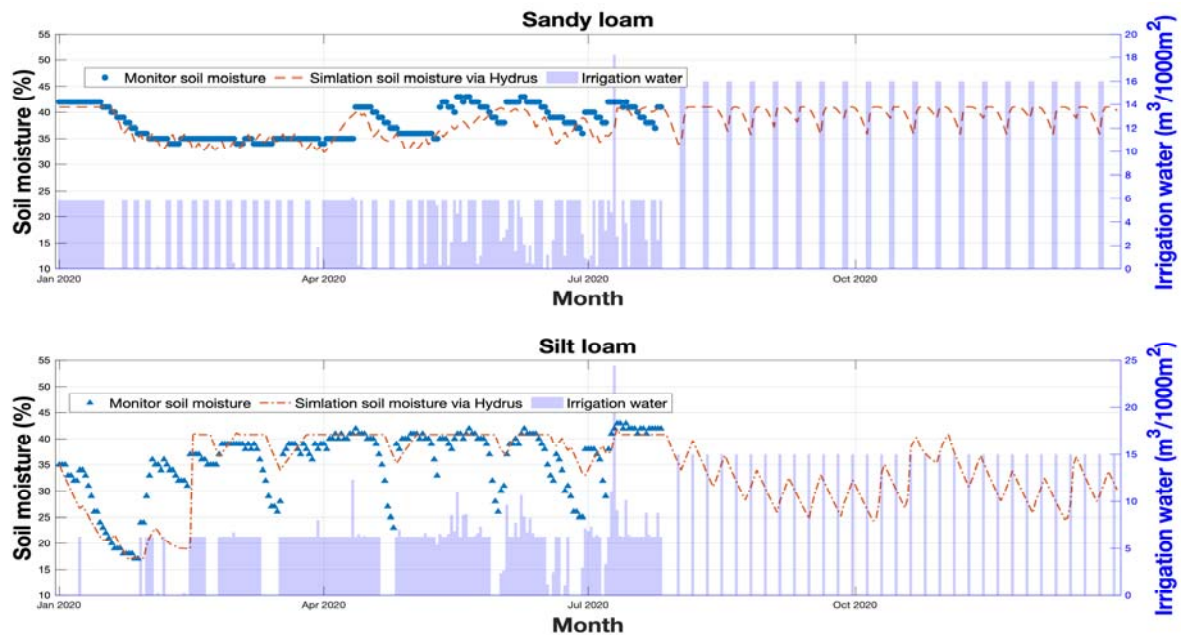
Figure 1. Comparison of soil moisture from past irrigation with an alternative irrigation model.
